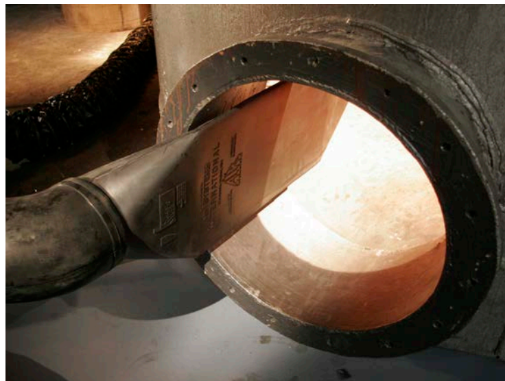
Tank 90° Elbow - 8" SV-90T
